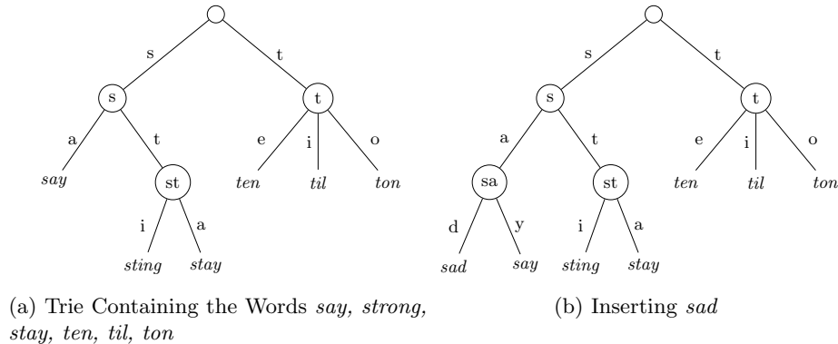
Fig. 2: An Example for an 26-ary Trie
